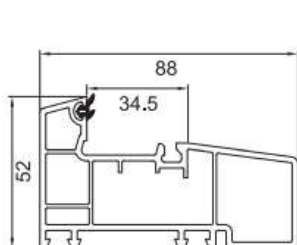
Fixed Frame FP-203-1 1.09Kg/m Length (m) 5.9 6 PCS (Per Pack)
