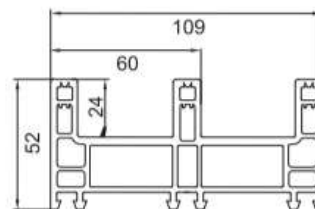
Frame FP-246H 1.72Kg/m Length (m) 5.9 4 PCS (Per Pack)
