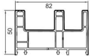
Frame FP-082 1.20Kg/m Length (m) 5.9 6 PCS (Per Pack)
