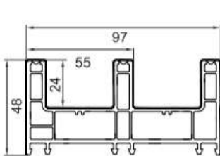
Frame FP-333 1.45Kg/m Length (m) 5.9 4 PCS (Per Pack)
