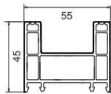
Frame FP-055 0.84Kg/m Length (m) 5.9 8 PCS (Per Pack)
