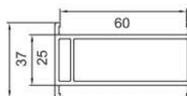
Coupling FP-049 0.68Kg/m Length (m) 5.9 6 PCS (Per Pack)
