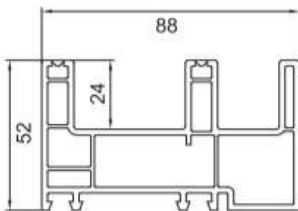
Frame FP-202-1 1.350Kg/m Length (m) 5.9 6 PCS (Per Pack)
