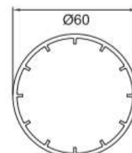
Coupling FP-013 0.62Kg/m Length (m) 5.9 6 Pcs (Per Pack)
