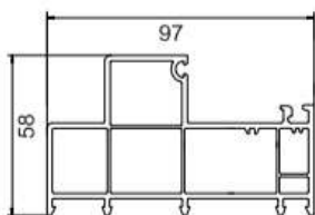
Frame FP-001 1.280 Kg/m Length (m) 5.9 4 Pcs (Per Pack)
