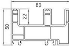
Frame FP-111 1.19Kg/m Length (m) 5.9 6 PCS (Per Pack)
