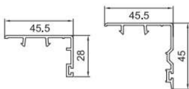
Inter lock FP-036 0.22Kg/m Length (m) 5.9 30 Pcs (Per Pack)
