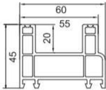
Frame FP-102 0.84Kg/m Length (m) 5.9 8 PCS (Per Pack)
