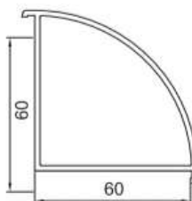
Coupling FP-051 0.68Kg/m Length (m) 5.9 4 Pcs (Per Pack)
