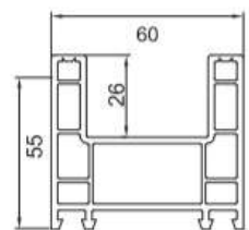
Frame FP-032-1 1.05Kg/m Length (m) 5.9 8 PCS (Per Pack)
