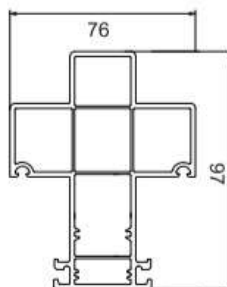
Mullion FP-002 1.440 Kg/m Length (m) 5.9 4 Pcs (Per Pack)
