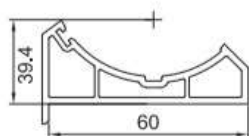
Coupling FP-090 0.53Kg/m Length (m) 5.9 6 Pcs (Per Pack)
