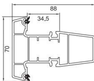
Fixed Mullion FP-204-1 1.17 Kg/m Length (m) 5.9 6 PCS (Per Pack)
