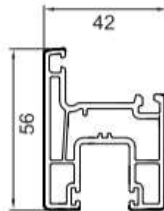
Window Sash FP-056 0.87Kg/m Length (m) 5.9 10 PCS (Per Pack)
