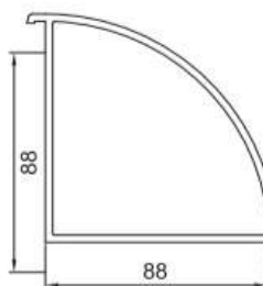
Coupling FP-080 1.19Kg/m Length (m) 5.9 4 Pcs (Per Pack)
