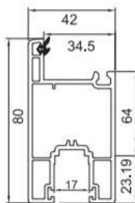
Door Sash FP-034 1.01Kg/m Length (m) 5.9 8 PCS (Per Pack)
