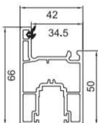
Window Sash FP-033 0.950Kg/m Length (m) 5.9 10 PCS (Per Pack)
