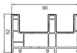
Frame FP-201 1.35Kg/m Length (m) 5.9 6 PCS (Per Pack)
