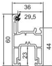
Sash FP-050-1 0.740Kg/m Length (m) 5.9 10 PCS (Per Pack)
