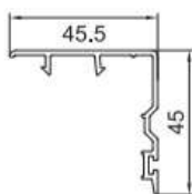
Inter lock FP-312 0.28Kg/m Length (m) 5.9 30 Pcs (Per Pack)
